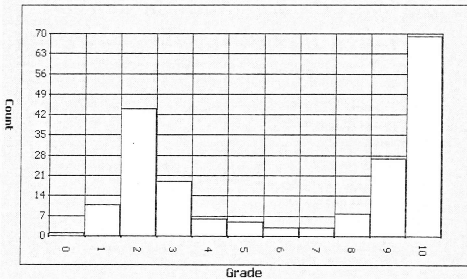
Grade Distribution for Written 2 Exam 1
